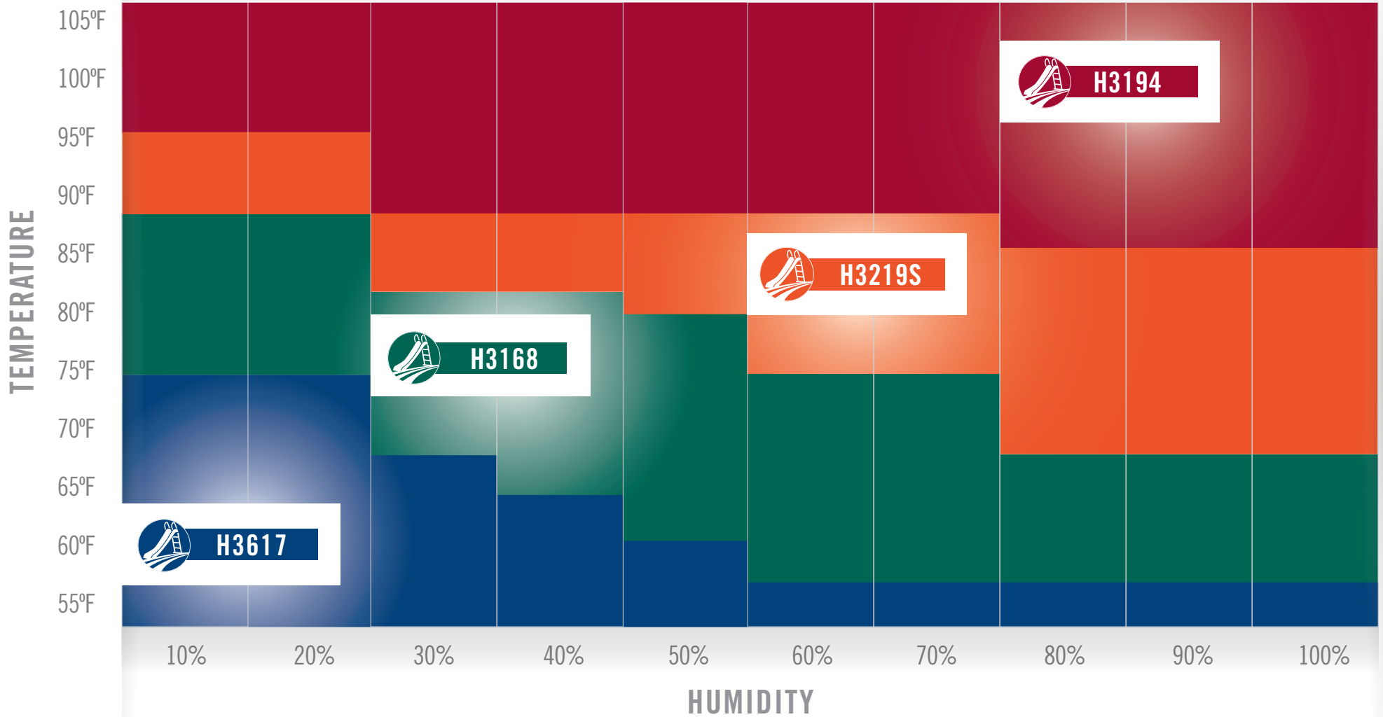
← FAST CURE RATE ACCELLA POLYURETHANE ALIPHATIC BINDER TEMPERATURE/HUMIDITY CHART SLOW CURE RATE →
